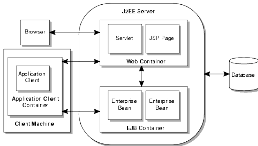
Figure (2.2): J2EE Container Types
