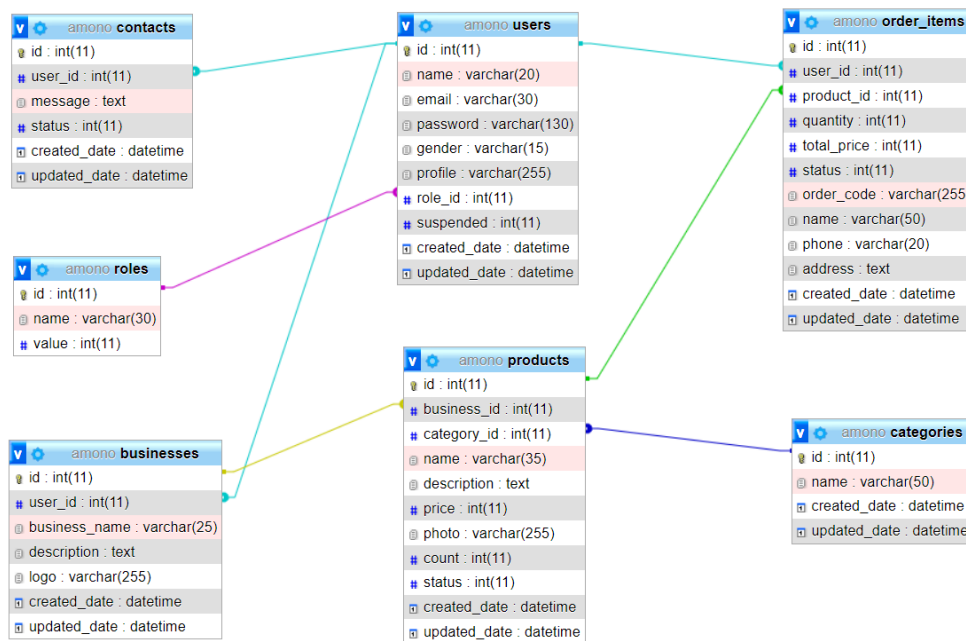
Figure (3.1): Entity Relationship Diagram for Amono Online Shop
