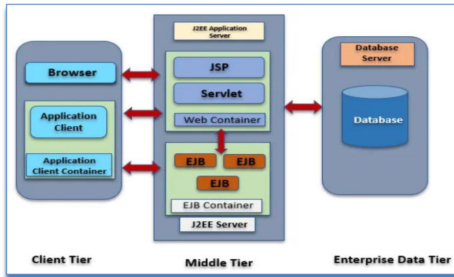
Figure (2.1) Architecture of J2EE
